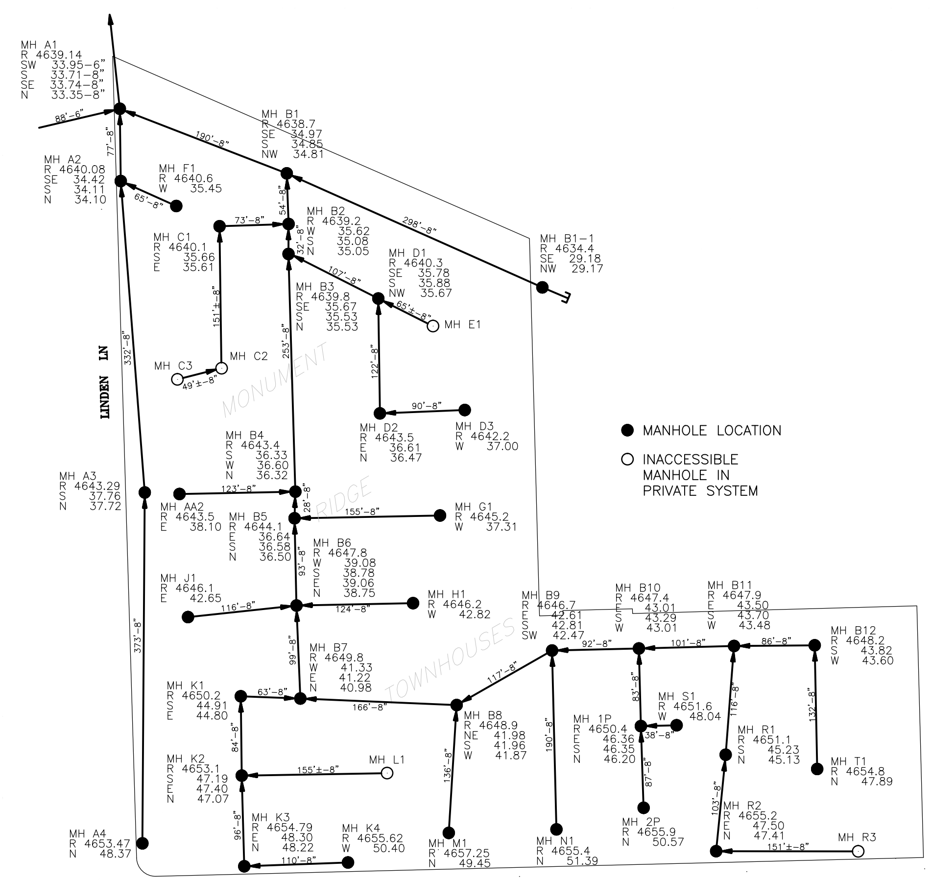
ENLARGED DETAIL OF MONUMENT RIDGE TOWNHOUSES SCALE: 1"=100'
